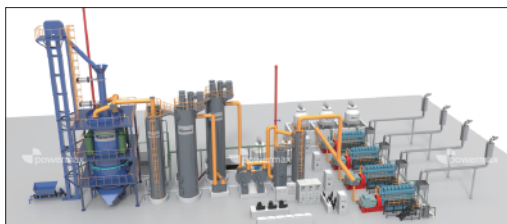
1.5MW Biomass Gasification Power Generation (Philippines)
